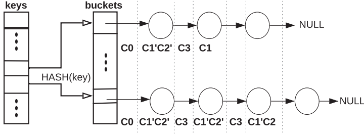
Fig. 5. Branch Outcome Stream Generation for two lookups in PHT. For this example, we assume a maximum of 4 nodes for each bucket and exactly two keys per node. For the bucket on top, there is a key match in the second node's first key. In the bottom bucket, a match has been found in the third node's second key. The branch outcome streams generated for each lookup are shown. For example, for the lookup in the top bucket, C0C1'C2'C3C1 is the branch outcome stream generated where C0–C3 are different branch pattern cases listed in Table 2.
