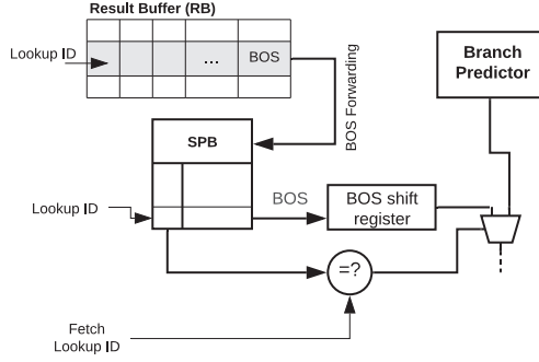
Fig. 6. BOS integration with the branch predictor.
