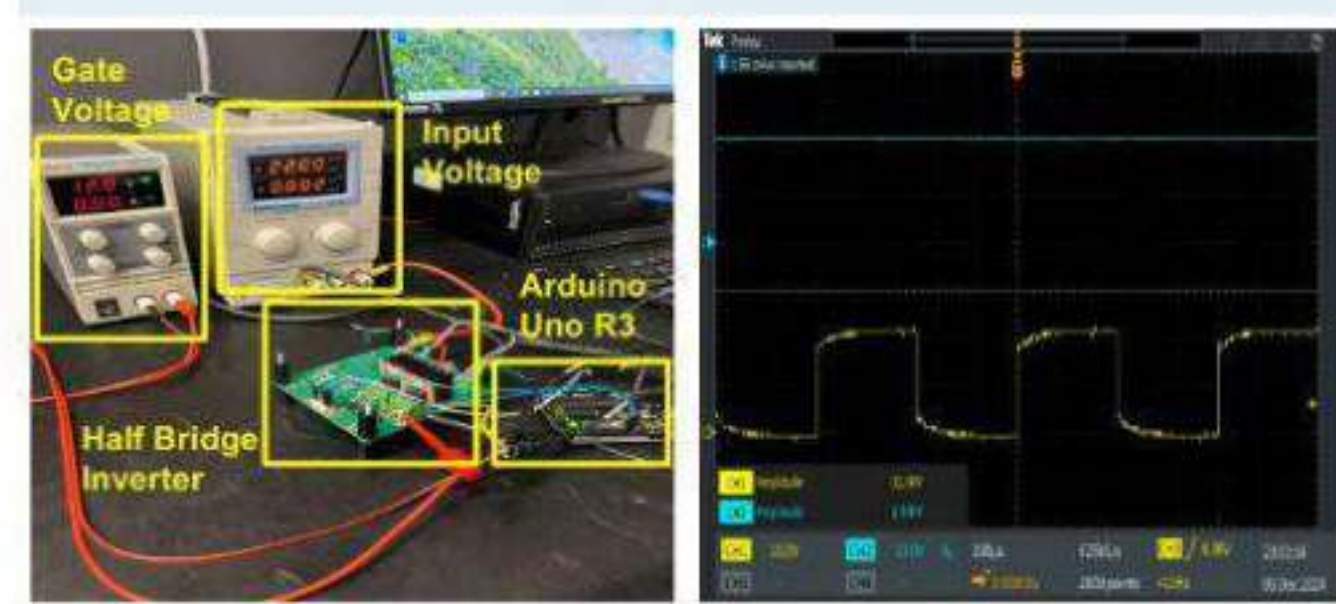
Inverter Stage
