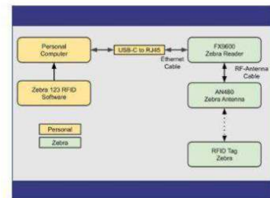
Figure 1: Block Diagram of RFID Testing Setup
