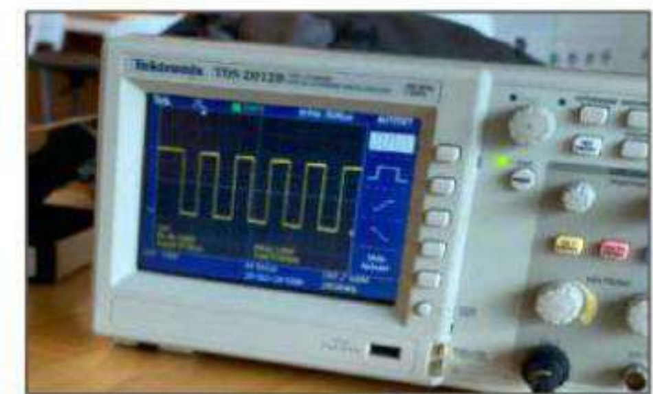
UART signal testing
