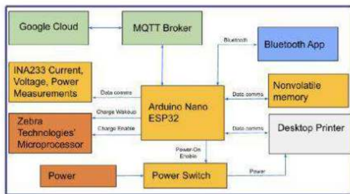
Fig. 4: Arduino Nano ESP32 Block Diagram
