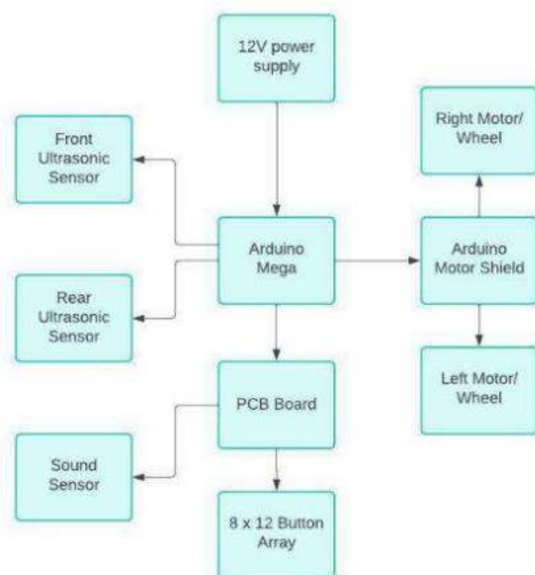
Fig. 4 Block Diagram of Robotoy
