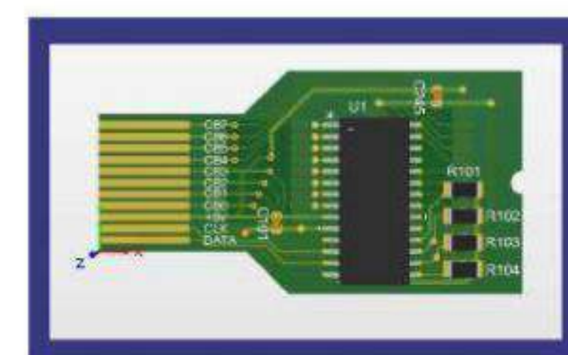
Horizontal CBIT Expander Card Layout
