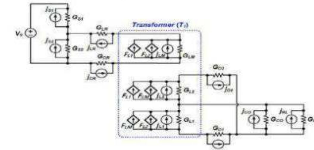
MNA Calculations of the LLC Converter
