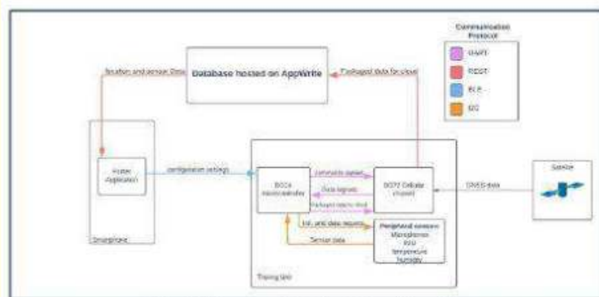
Block Diagram of Project Functionality
