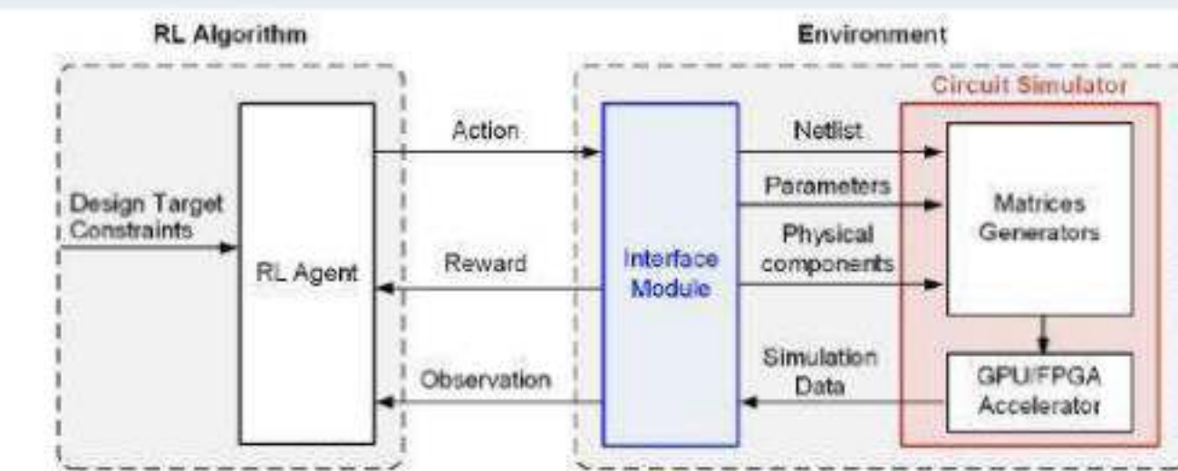
Architecture of the RL-based PEDA Tool
