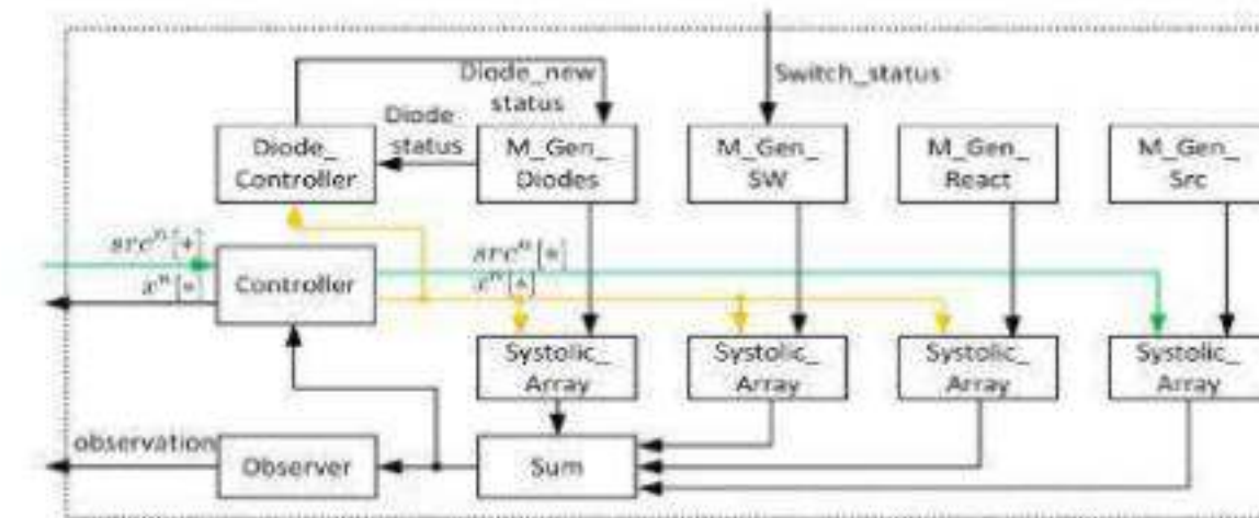
Systolic MNA Calculations Flow Chart
