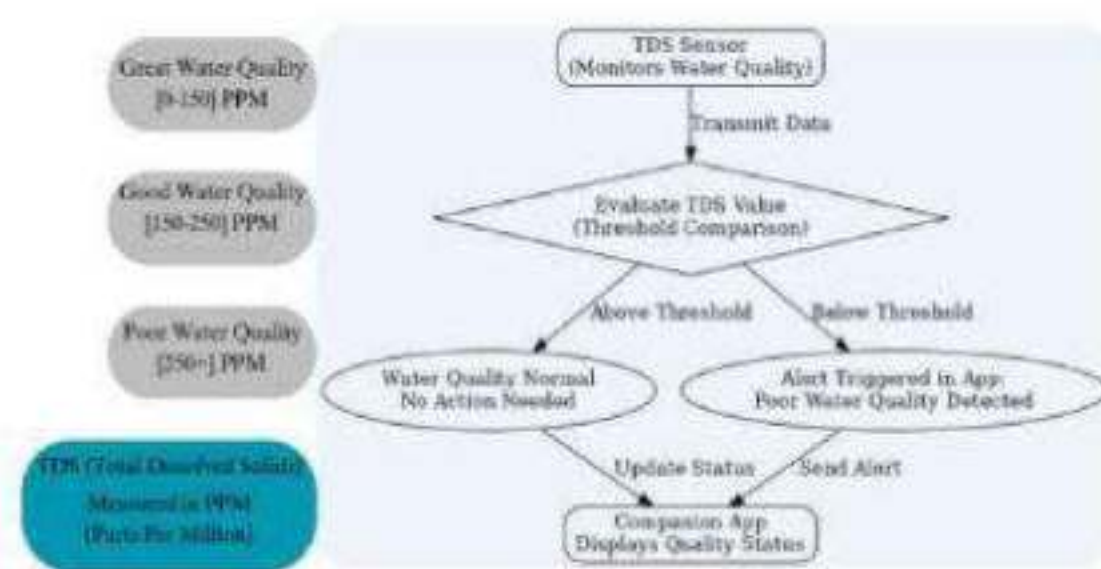
Fig 4: TDS Sensor Water Quality Extraction Flowchart
