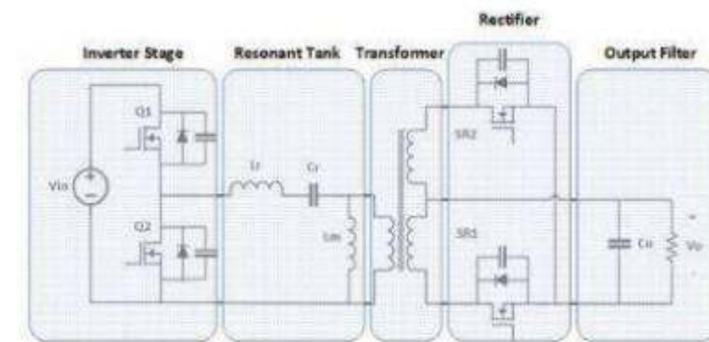
Half-Bridge LLC Resonant Converter
