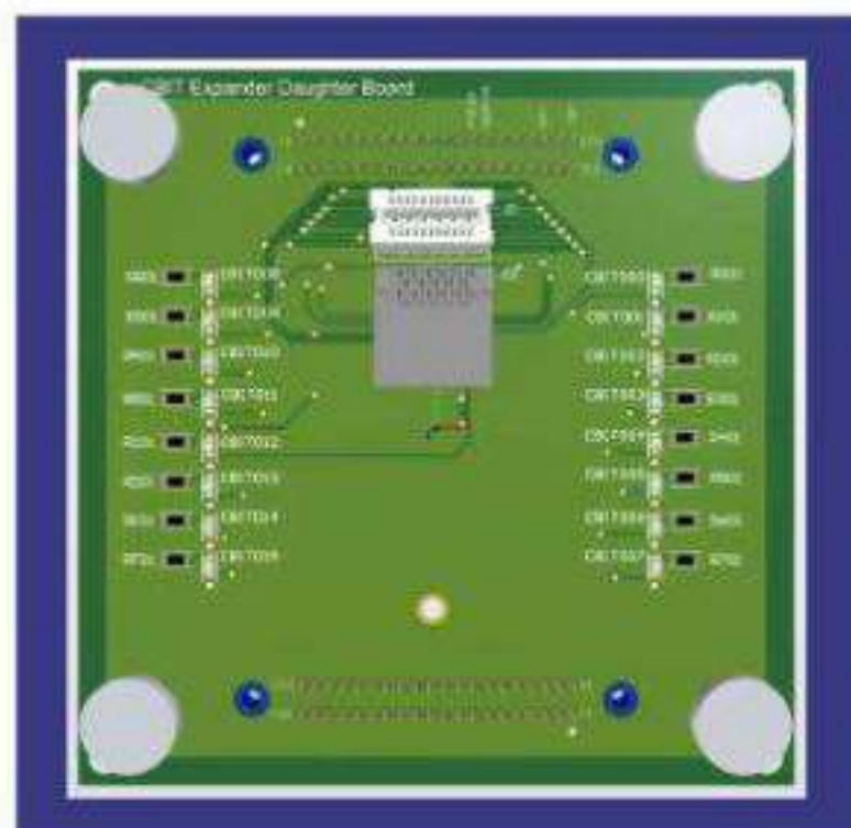
CBIT Expander Daughter Board Layout
