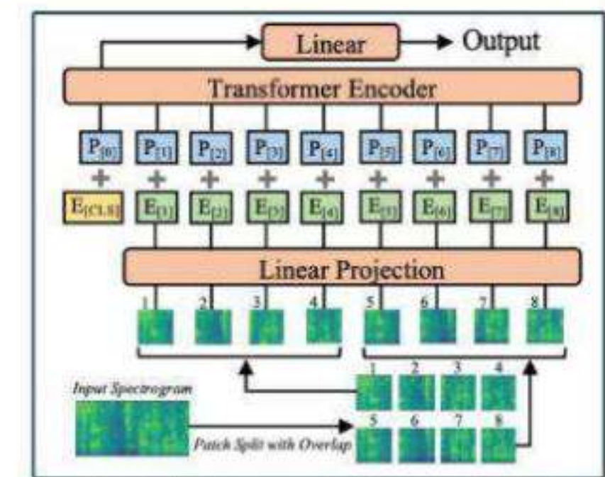
Fig. 1: Audio Spectrogram Transformer architecture
