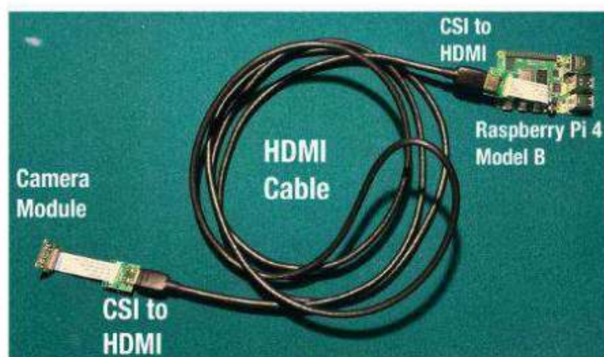
Current design and testing setup
