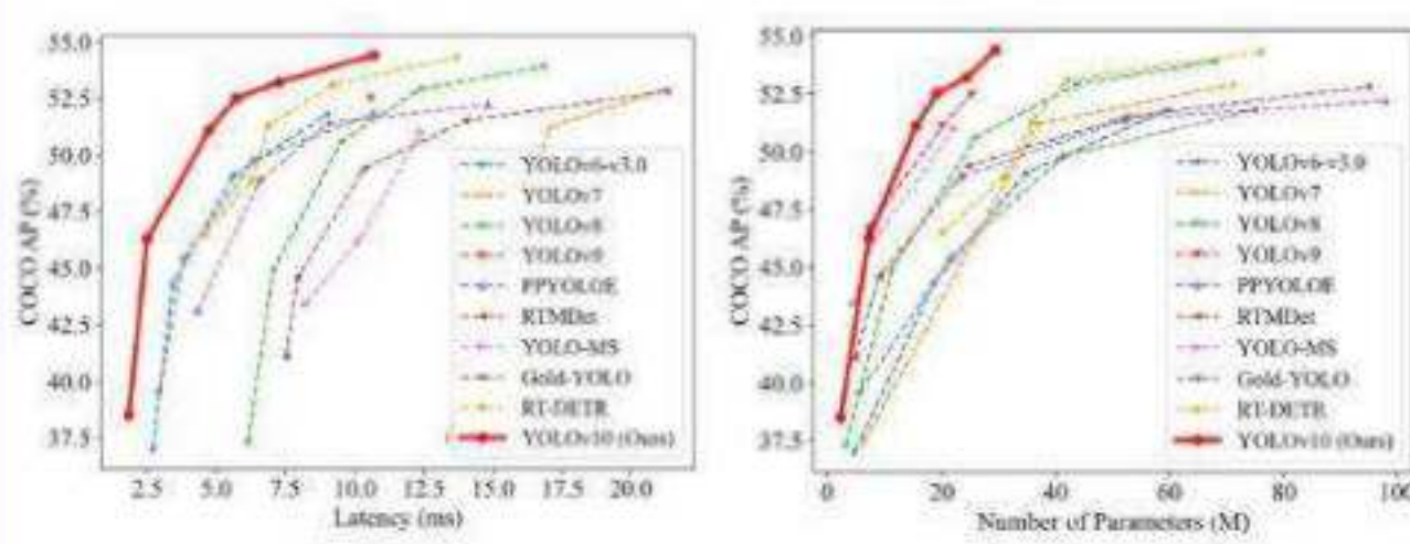
YOLOv10 Compared to Other Models
