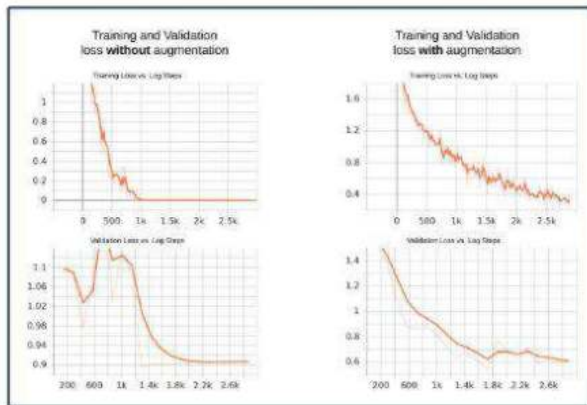
Fig. 4: Comparison of loss trends between non-augmented data and augmented data
