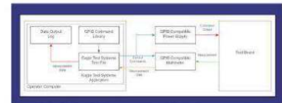
Simplified Block Diagram for GPIB Command Library
