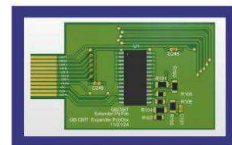
Vertical CBIT Expander Card Layout
