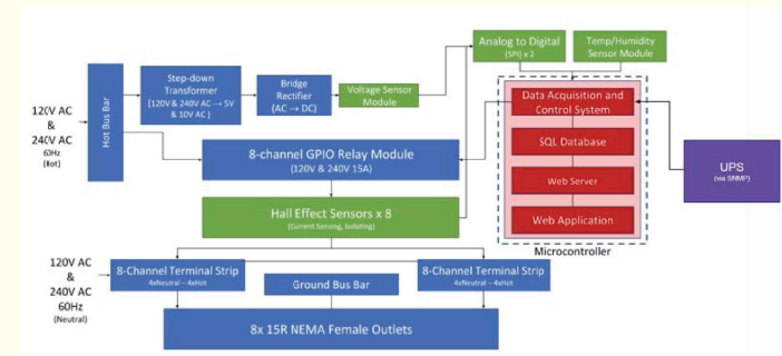
Fig 4: Updated block diagram for the product. Capabilities for UPS communication as well as 240v have been added.
