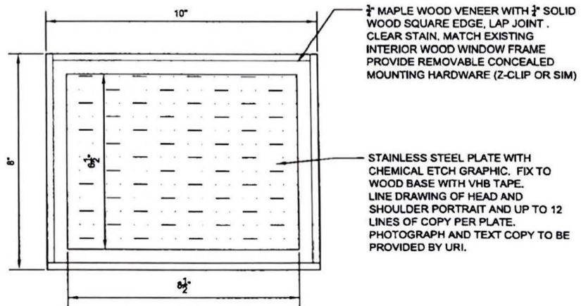
TYPICAL SIGN PANEL DETAIL
