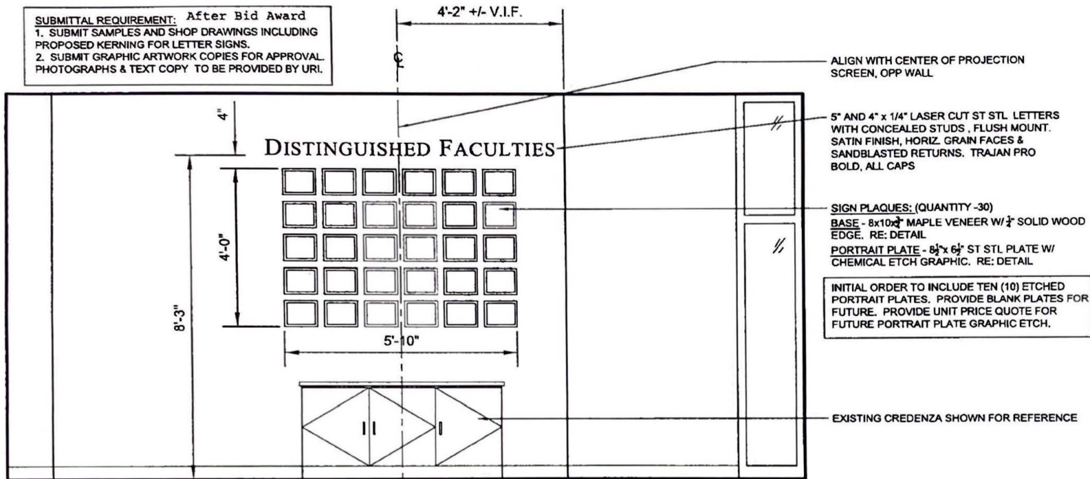
ELEVATION - NORTH WALL SCALE: 1/2" = 1'-0"
