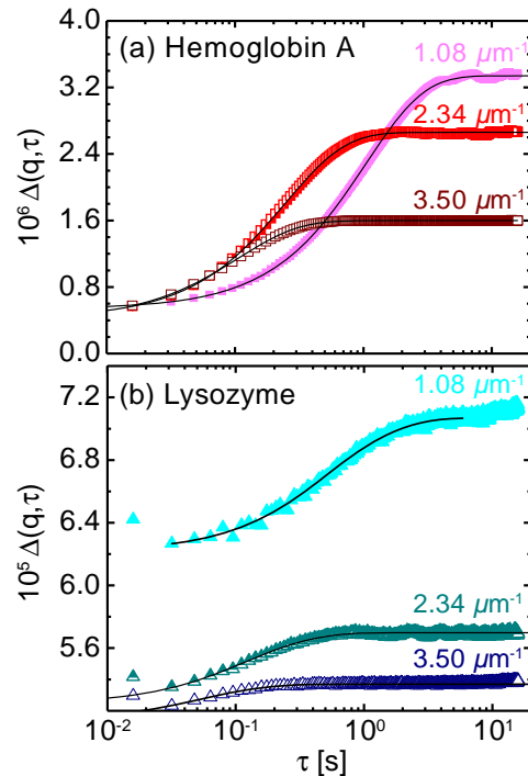
FIG. 3. (Color online) Structure function \Delta as a function of lag time \tau at three wave vectors q , indicated in the plots, for solutions of (a) hemoglobin A at a concentration of 50 \text{mg ml}^{-1} and (b) lysozyme at a concentration of 103 \text{mg ml}^{-1} . Lines are best fits to Eq. (1).
