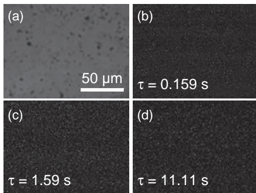
FIG. 1. (a) Representative bright-field micrograph of a hemoglobin A solution with a concentration of 50 \text{mg ml}^{-1} . (b)–(d) Representative subtractions of two images at lag times \tau , as indicated in the panels. The scale bar for all images is shown in (a).
