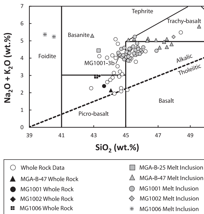
Figure 1. \text{Na}_2\text{O} + \text{K}_2\text{O} versus \text{SiO}_2 plotted with the alkali-tholeiite basalt line from MacDonald and Katsura [1965] and applicable rock types. Mangaia melt inclusions are plotted as gray symbols and were corrected for olivine addition or subtraction (following the methods outlined in Jackson et al. [2012]) to be in equilibrium with their host olivine (see supporting information Table S5 for olivine-corrected concentrations). The whole rocks hosting the respective melt inclusions are plotted as the same symbol as the melt inclusions, but in black. Previously published whole rock data are shown as white circles and were obtained from Georoc [Sarbas, 2008]. One sample (M17) from Woodhead [1996] contains anomalously low \text{Na}_2\text{O} . We argue that this is a result of significant alteration, which is supported by the high loss on ignition (LOI) of 9.33% for this sample; we have removed this sample from the figures. Whole rock data for MGA-B-25 is not available. Samples from this study plot in the alkalic field.
