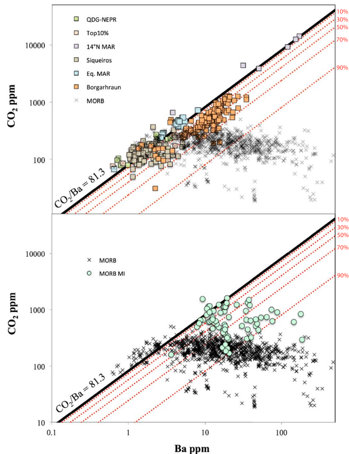
Figure 4. (a) CO 2 versus Ba for suites of vapor-undersaturated melt inclusions and mid-ocean ridge basalt (MORB; squares, summarized in Hauri et al., 2017) together with data from globally distributed MORB (crosses). (b) Same diagram as panel (a) showing only MORB glasses and MORB melt inclusions from Shaw et al. (2010), Wanless & Shaw (2012), Helo et al. (2011), and Wanless et al. (2014, 2015). The heavy black line represents the average CO 2 /Ba (81.3) derived from the CO 2 /Ba ratio of undersaturated samples. Red dashed lines with labels indicate the extent of CO 2 degassing.
